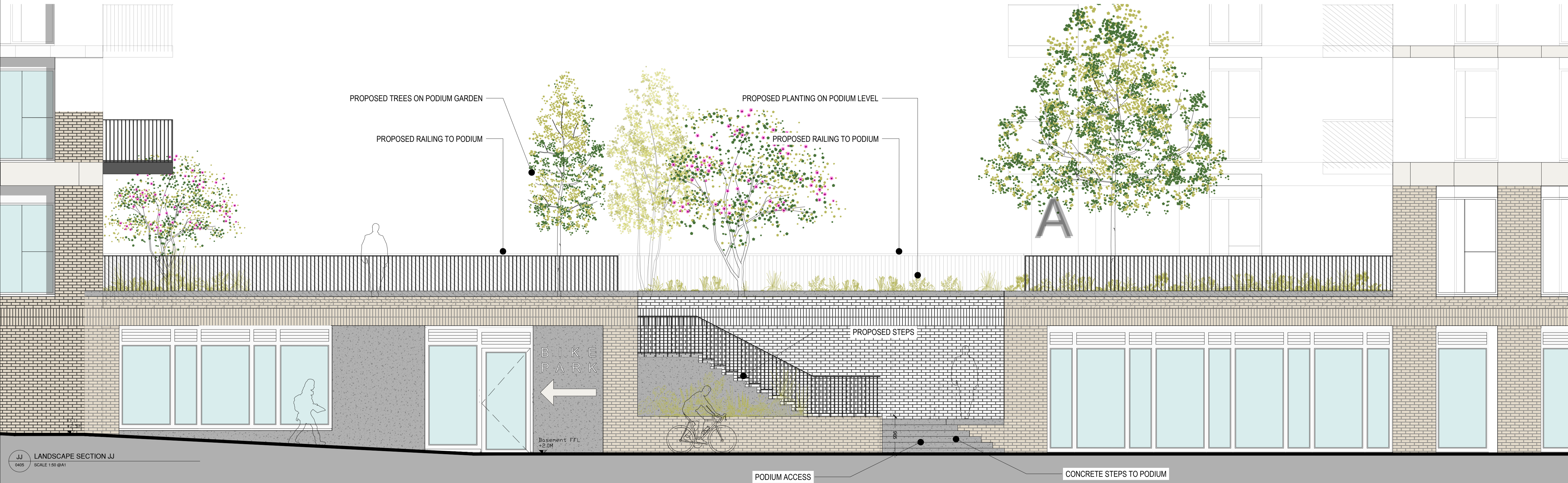
II LANDSCAPE SECTION II SCALE 1:50 @A1
