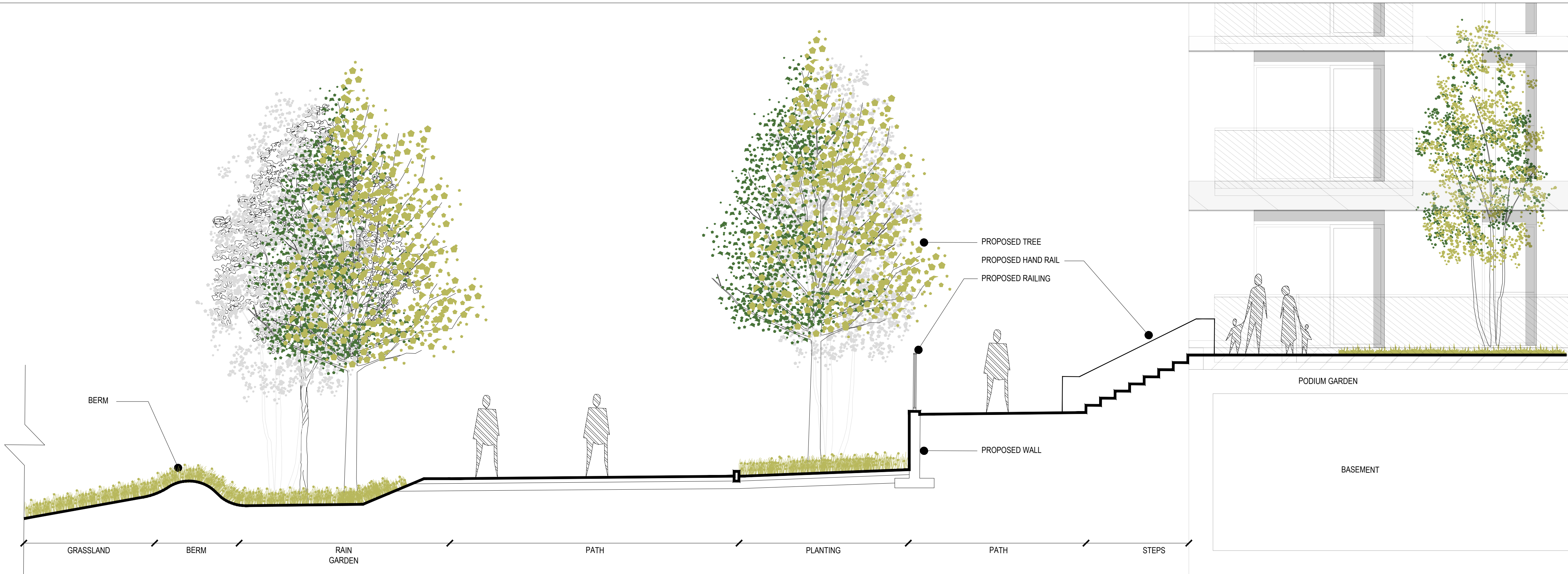
CC LANDSCAPE SECTION CC 0402 SCALE 1:50 @A1
