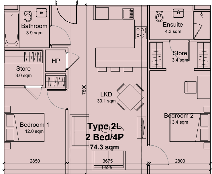
Unit type 2L: 2 Bed / 4 Persons apartment
