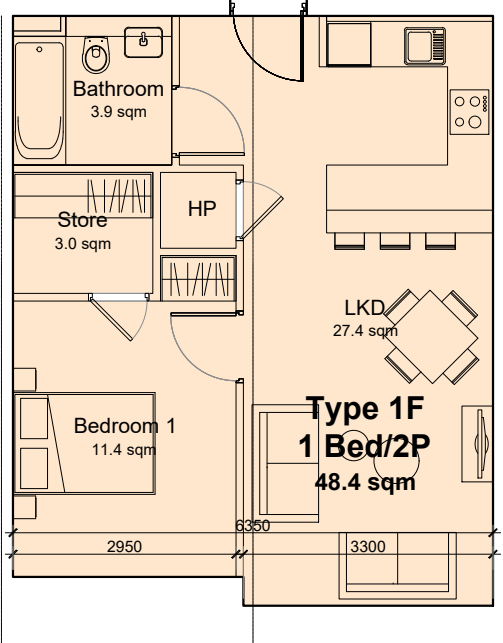
Unit type 1F: 1 Bed / 2 Persons apartment
