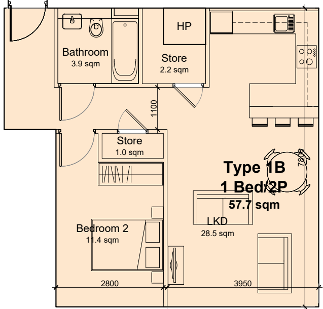
Unit type 1B: 1 Bed / 2 Persons apartment
