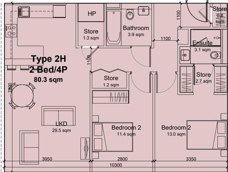
Unit type 2H: 2 Bed / 4 Persons apartment
