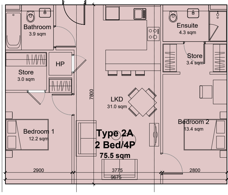
Unit type 2A: 2 Bed / 4 Persons apartment
