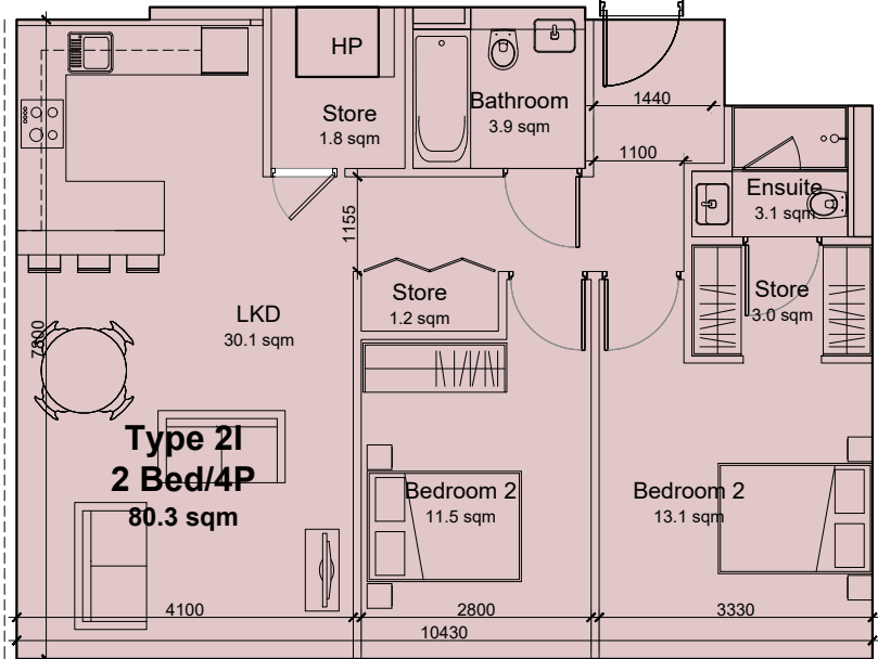
Unit type 2I: 2 Bed / 4 Persons apartment
