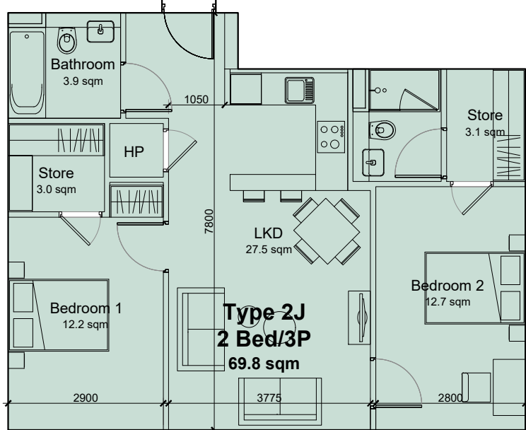
Unit type 2J: 2 Bed / 3 Persons apartment
