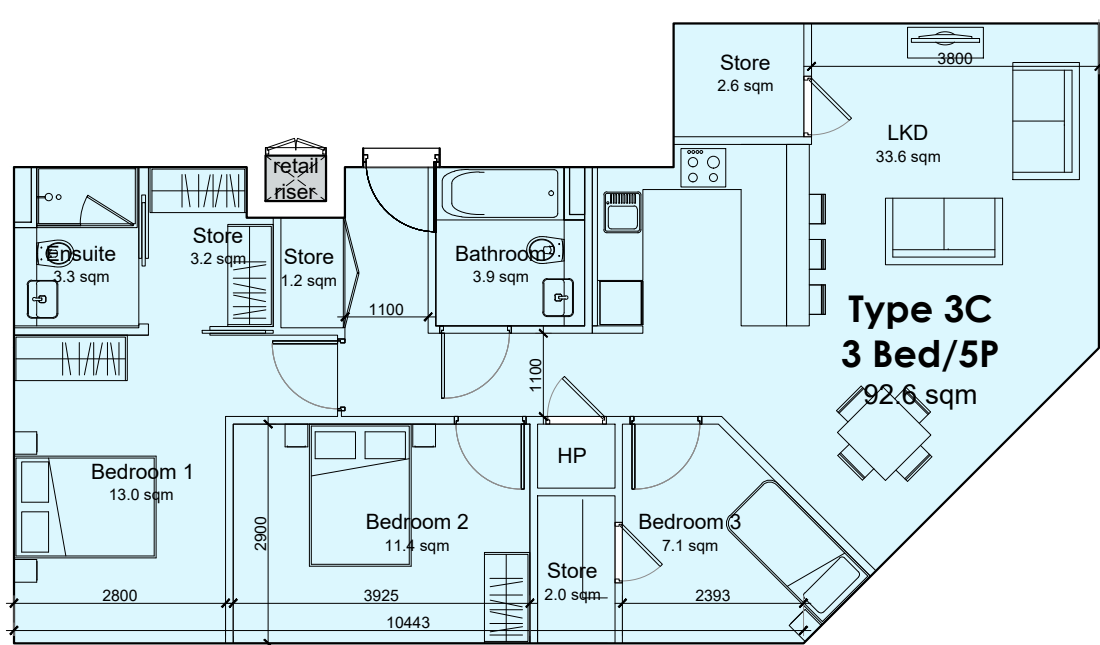
Unit type 3C: 3 Bed / 5 Persons apartment
