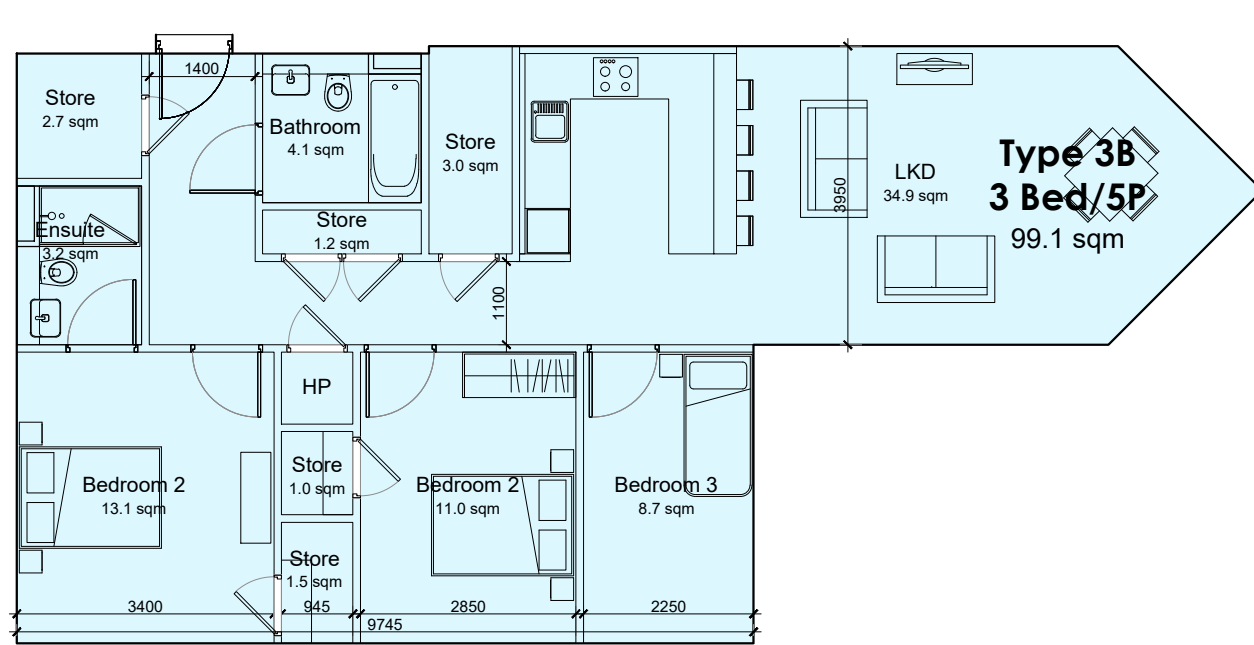
Unit type 3B: 3 Bed / 5 Persons apartment
